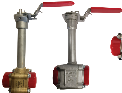
Part # WC-C44-1166-PMSE-1
